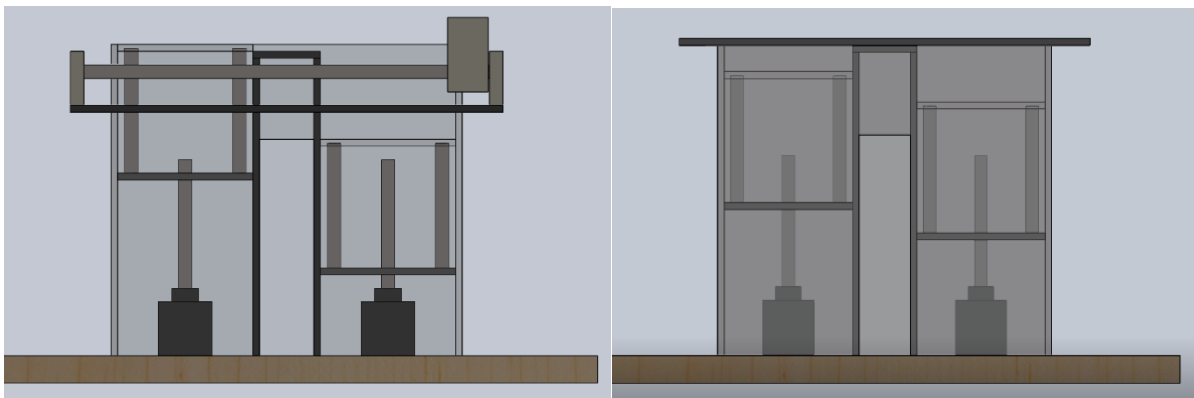
Figure 17a Front View of Sand Containers
