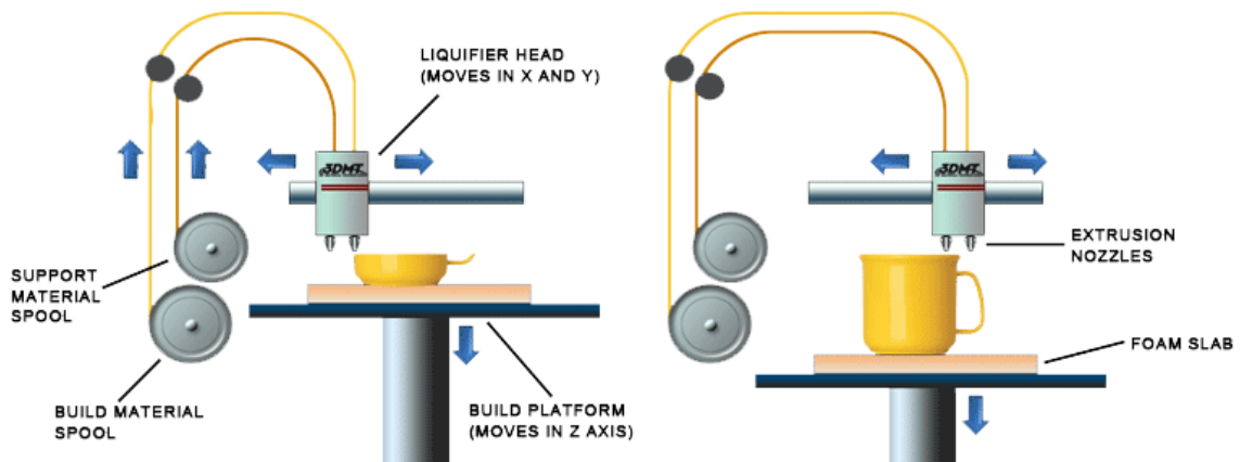
Figure 4 Fused Deposition Modeling Process
