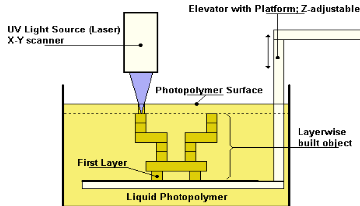
Figure 3 Stereo lithographic Process
