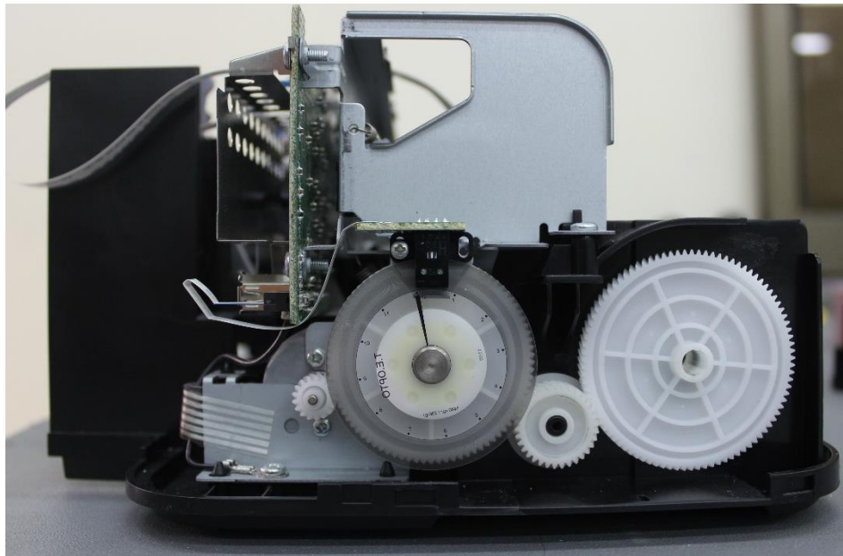
Figure 23 Assembly (Motor / Encoder / Roller)
