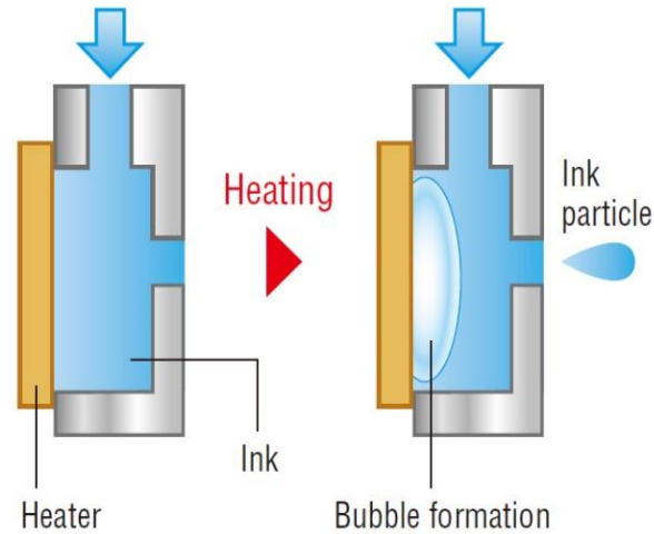
Figure 13 Thermal Print Head Working Mechanism
