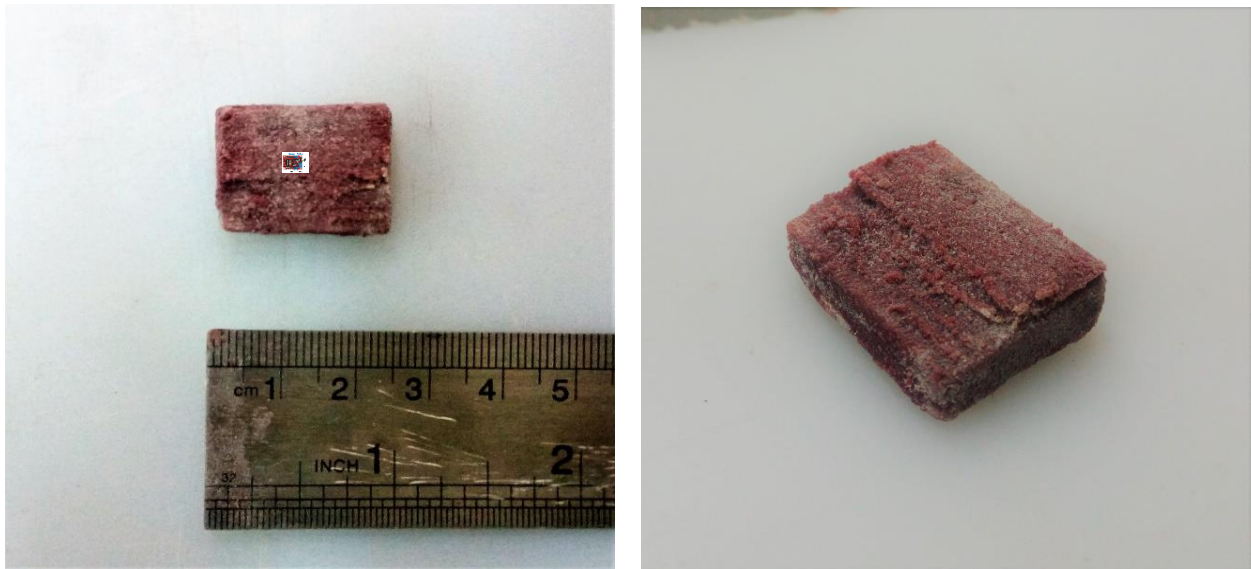
Figure 26 3D Printed Sand Mold Sample
