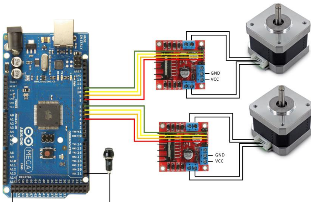
Figure 20 Wired Configuration For Controlling Sand Beds
