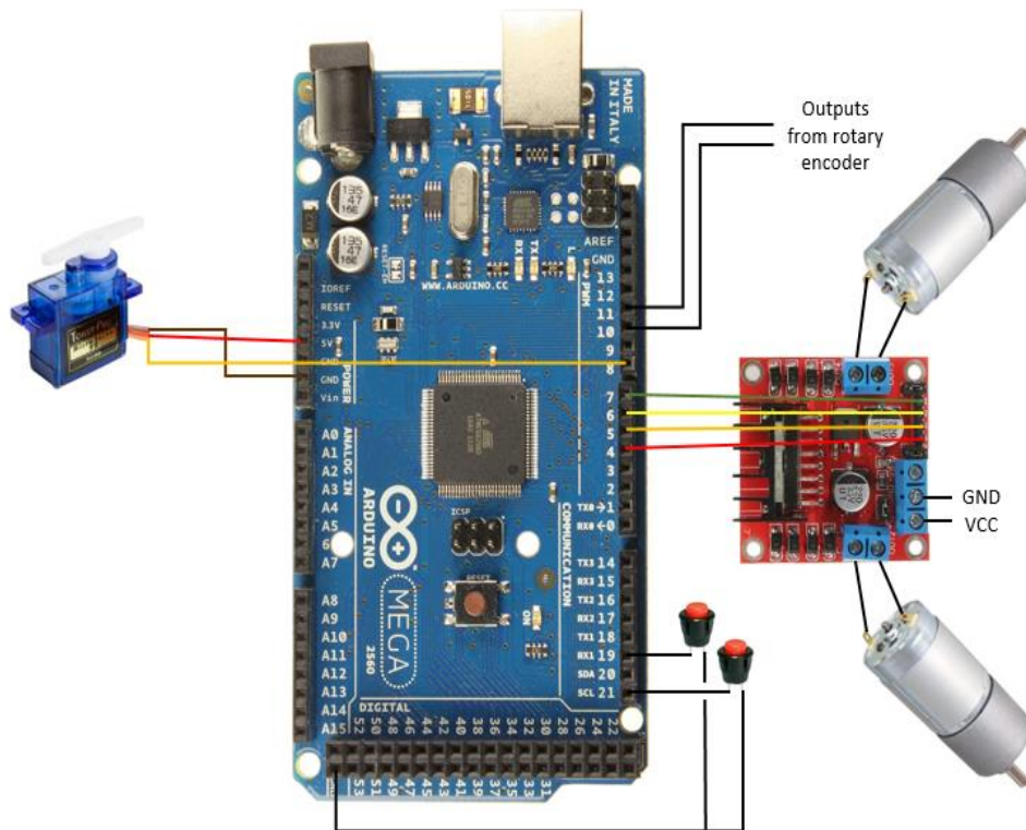
Figure 24 Print Mount Control Circuit Wiring
