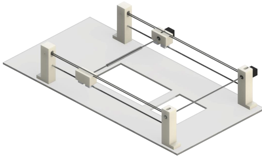
Figure 21 Rendered 3D Model of Recoater
