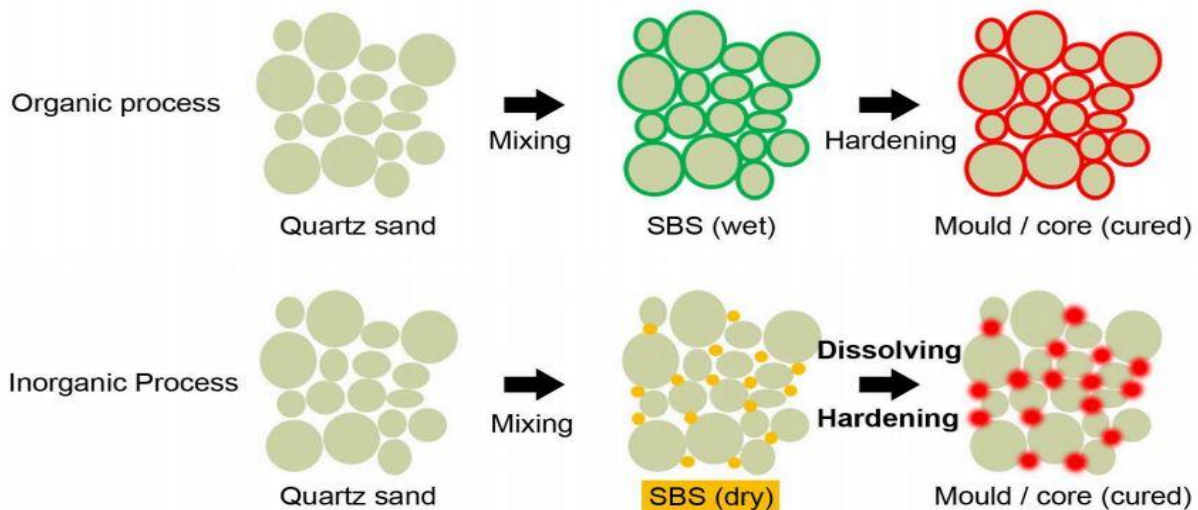
Figure 11 Difference between organic and inorganic binder processes
