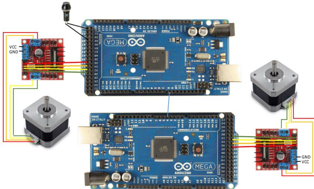
Figure 22 Recoater Control Circuit Wiring
