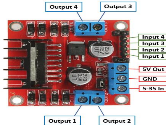
Figure 19 L298N Motor Driver Pinout Diagram
