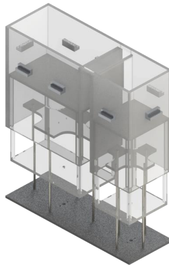
Figure 17 Complete 3D View of Sand Beds
