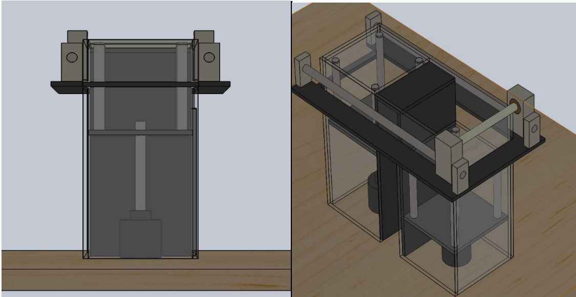
Figure 17b Side View
