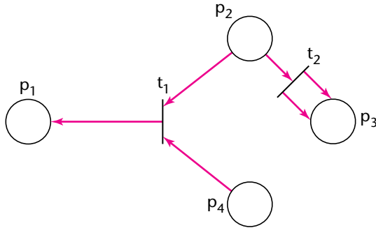
FIGURE 12.18 A Petri net.
