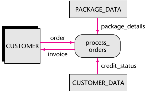
FIGURE 12.2 The data flow diagram for Sally's Software Shop: first refinement.
