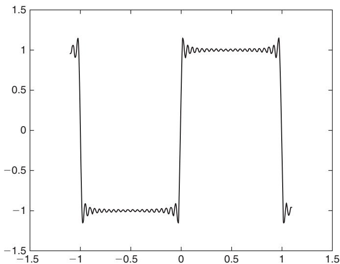
FIGURE 8.3 Fourier series: The Gibbs phenomenon.
