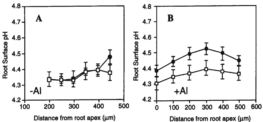
Fig. 1. Influence of \text{Al}^{3+} exposure on rhizosphere pH along the surface of A. thaliana root tips in wild type ( \square ) and alr-104 mutant resistant to Al ( \bullet ). The mutant did not show enhanced root organic acid release in the absence (A) or presence (B) of 300 \mu\text{M} \text{AlCl}_3 (Source: Degenhardt et al. 1998)
