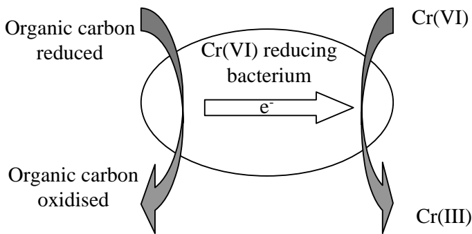
Fig. 4. Bacterial direct enzymatic reduction of Cr(VI)
