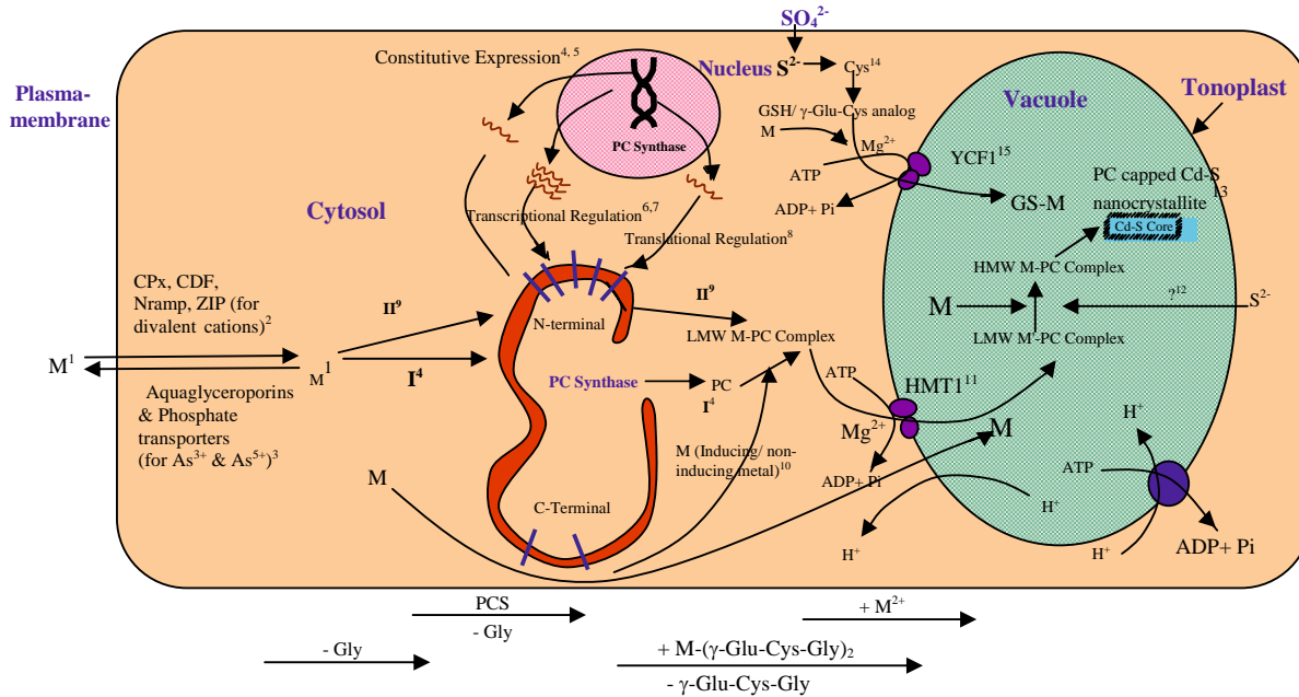
Fig. 1: Schematic representation of PC mediated metal detoxification. Metal or metalloid enters into the cytosol by different type of transporters. Within the cytosol metal activates PCS either by direct interaction (I) or by interaction of metal-glutathione complex with the enzyme (II). PCS enzyme may be present constitutively or may be regulated at the level of transcription or translation. PC-metal complex (LMW) thus formed is transported into vacuole by ATP energized ABC type transporters. Inside vacuole HMW complexes are formed from LMW complexes by incorporation of sulfide ions. HMW complexes may be stabilized in the form of nanocrystallites having metal-sulfide core capped by PCs. Superscript denote references which are given as follows. 1 - Zenk et al., 1996, 2 - Hall and Williams, 2002, 3 - Abedin et al., 2002, 4 - Grill et al., 1989, 5 - Vatamaniuk et al., 1999, 6 - Clemens et al., 1999, 7 - Lee and Korban, 2001, 8 - Heiss et al., 2003, 9 - Vatamaniuk et al., 2000, 10 - Maitani et al., 1996, 11 - Ortiz et al., 1992, 1995, 12 - Mehra and Tripathi, 2000, 13 - Dameron et al., 1990, 14 - Saito, 2004, 15 - Li et al., 1997
