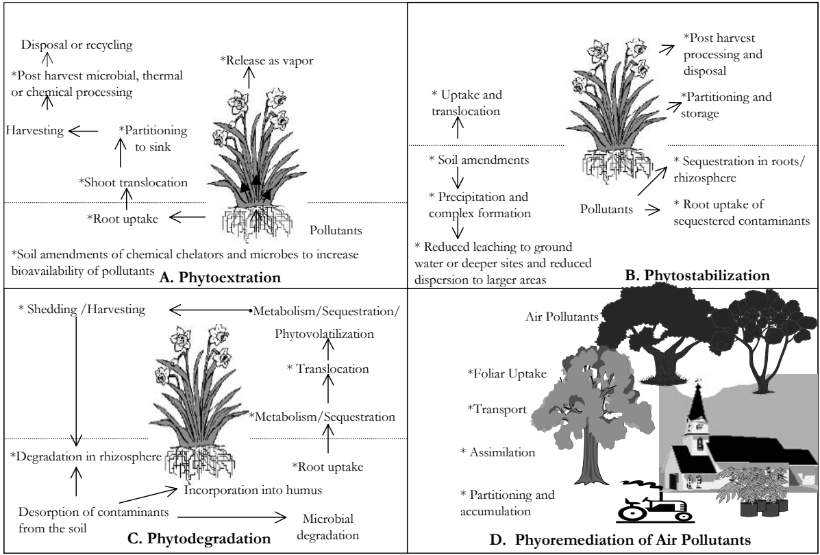
Fig. 1. Phytoremediation types and postulated sites for biotechnological interventions A. Phytoextraction / Phytovolatilization, B. Phytostabilization, C. Phytodegradation, D. Phytoremediation of air pollutants; *Sites for Biotechnological input
