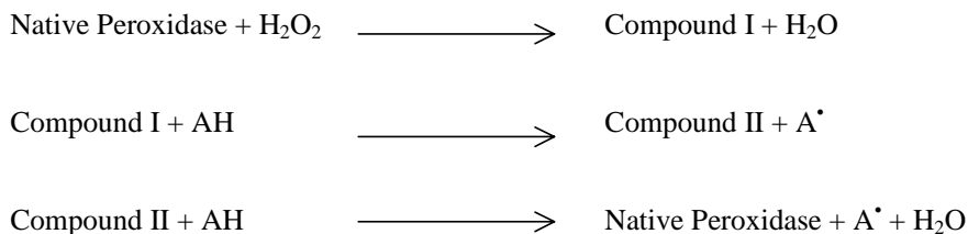
Fig. 4. Simplified catalytic cycle for heme peroxidases [AH: reducing substrate; A • : free radical (oxidised substrate)]
