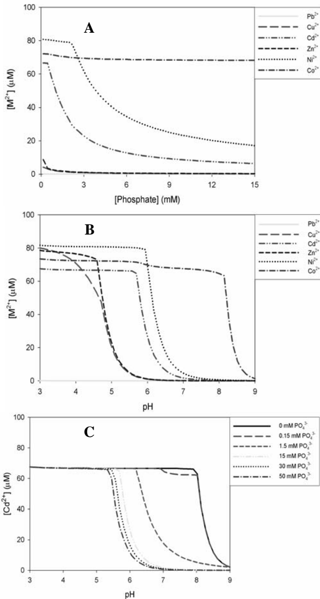
Fig. 1. Effect of phosphate concentration (A), pH (B), and interactions of phosphate and pH (C) on solution-phase, ionic metal ( [M^{2+}] ) and cadmium ( [Cd^{2+}] ) concentrations as predicted by MINEQL+ geochemical modeling software (Environmental Research Software, Hallowell, ME, USA) in Bushnell-Haas broth (Difco, Sparks, MD) amended with 100 \mu M total lead, copper, cadmium, zinc, nickel, or cobalt. When prepared according to the manufacturer's specifications, Bushnell-Haas broth contains 15 mM pH and has a pH of 7.0 \pm 0.2 . The pH of the medium in (A) was set at 6.5
