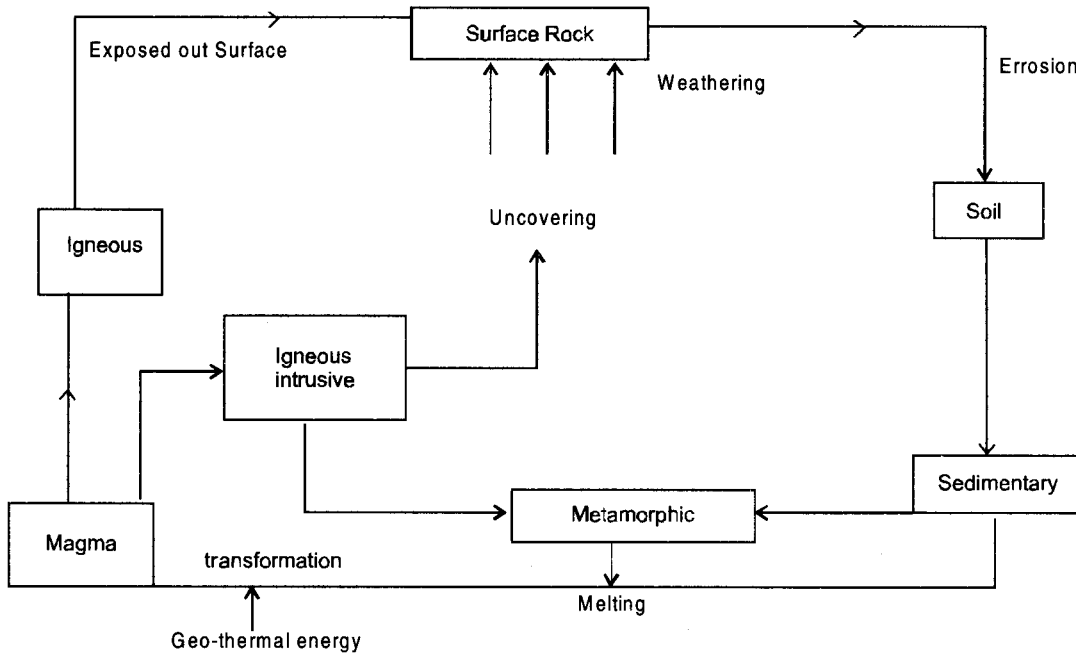
Geological Cycle
