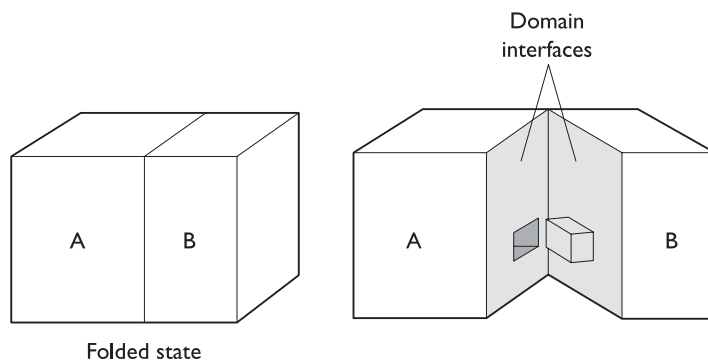
Fig. 6.18 Domain interface of a two-domain protein. In the folded state, interactions between the domains are inaccessible to the solvent. There is a free energy cost to exposing the domain interface to solvent, even if the domains themselves remain folded. The domain interface consists of two geometrically complementary surfaces.
