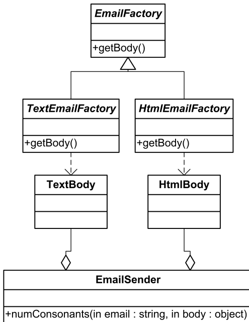
Figure 7.2. The Spam Factory
