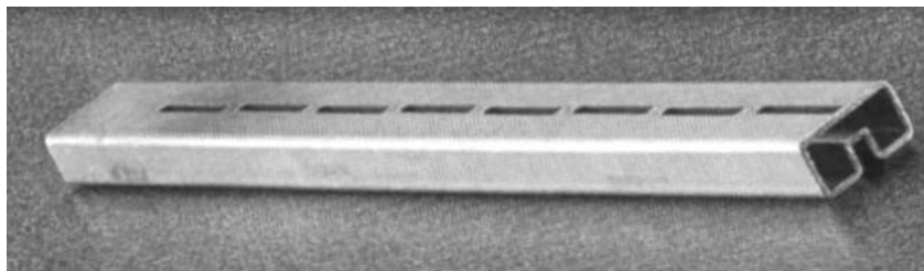
Figure 11.2 An example of an extruded waveguide profile which can be used for antenna applications [3].
