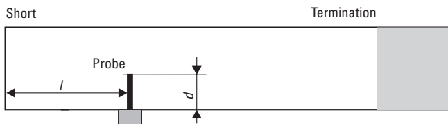
Figure 17.2 The basic configuration used in the tests was initially a probe-fed S or Ku-band rectangular waveguide, which was terminated with microwave absorbing material. The position of the short circuit (marked as l ) and the probe length d were used as input variables.
