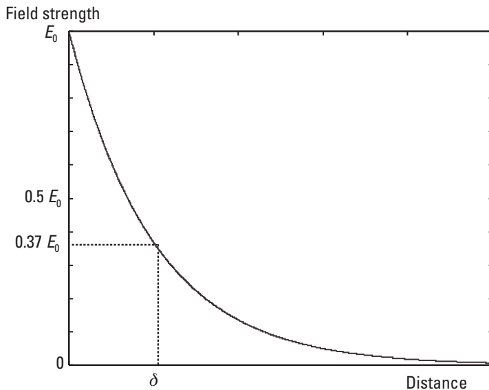
Figure 1.7 Electromagnetic wave penetration in a medium. The distance \delta is the penetration depth, where the amplitude has decreased by 1/e or about 8.7 dB from the initial value.
