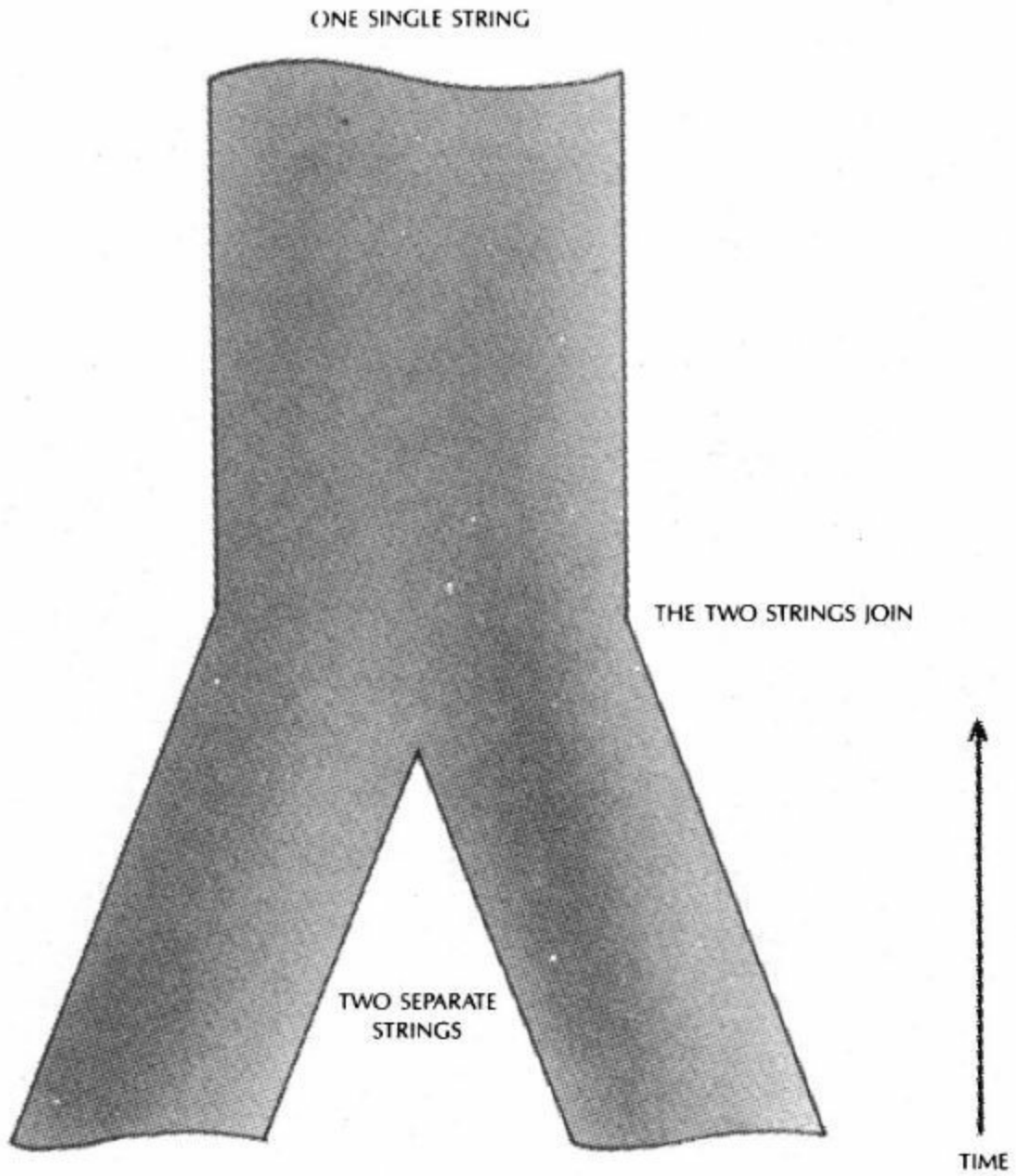
WORLD-SHEET OF TWO OPEN STRINGS JOINING
