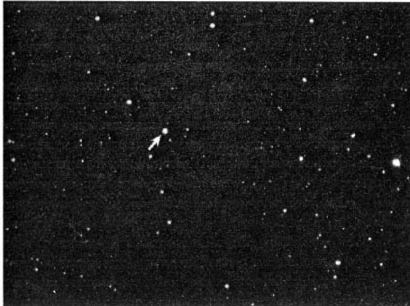
FIGURE 6.2 The brighter of the two stars near the center of the photograph is Cygnus X-1, which is thought to consist of a black hole and a normal star, orbiting around each other.
